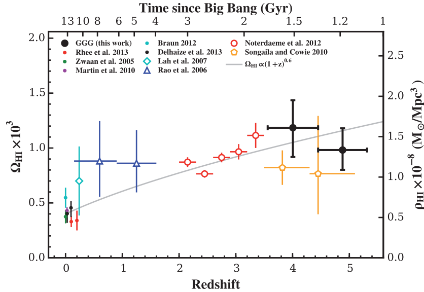
Figure 12. Measurements of \Omega_{\text{HI}} at different redshift, from Zwaan et al. (2005), Rao, Turnshek & Nestor (2006), Lah et al. (2007), Braun (2012), Martin et al. (2010), Noterdaeme et al. (2012), Rhee et al. (2013), Delhaize et al. (2013) and S10 (see Table 5). We do not show the measurement using SDSS QSOs by Prochaska & Wolfe (2009); it is consistent with the measurement by Noterdaeme et al. (2012), who use a superset of SDSS QSOs. We also do not show the Péroux et al. (2003) and Guimarães et al. (2009) results, which have a large overlap with the QSO sample used by S10 and are consistent with that measurement. Finally, for clarity, we do not show the measurements at lower redshift from Freudling et al. (2011) and Meiring et al. (2011); they are consistent with the plotted values. All measurements have been converted to the same cosmology ( h = 0.7 , \Omega_{\text{m}} = 0.3 , \Omega_{\Lambda} = 0.7 ) and include H I mass only, with no contribution from helium or molecular hydrogen.
